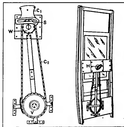
Fig. 5—Views of Perfect window regulator
